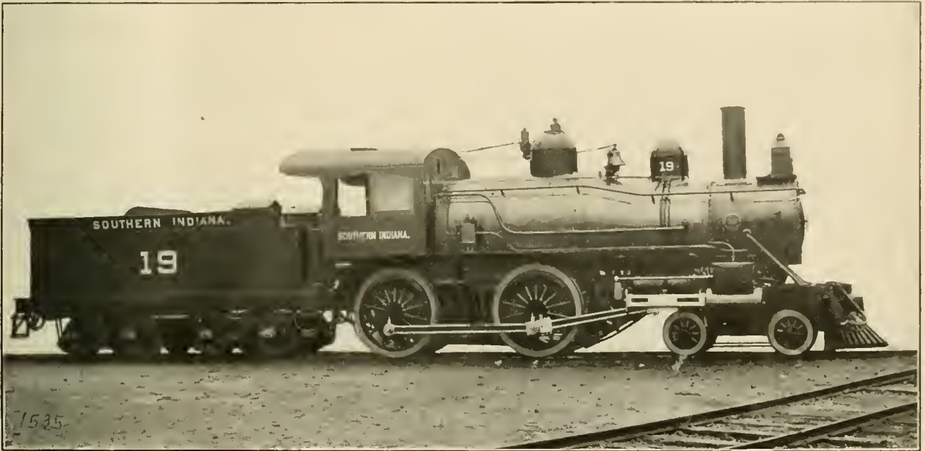
BALDWIN SIMPLE EIGHT-WHEELER FOR SOUTHERN INDIANA.
